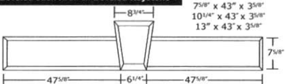
Beveled Jack Arch w/ Beveled Keystone
