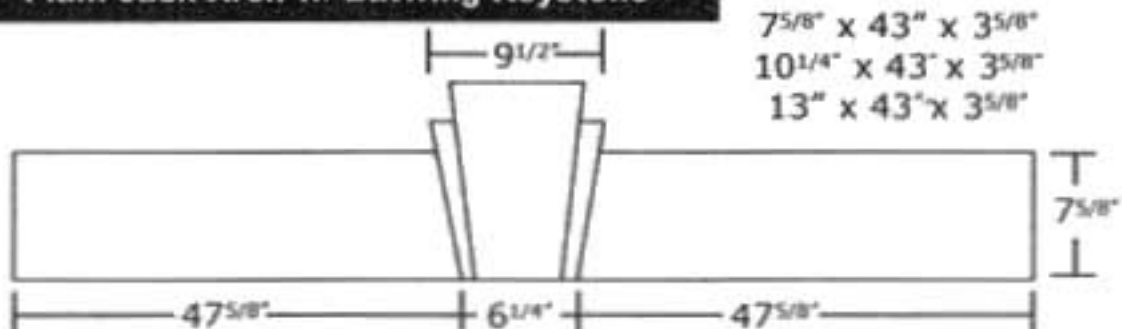
Plain Jack Arch w/ Batwing Keystone
